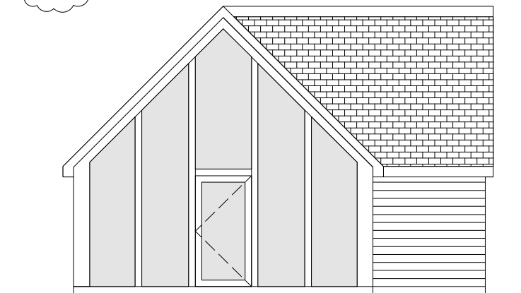
North-East Elevation
